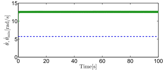
Fig. 4. Evolution of \theta (—) and the minimum value required to maintain contact (- - -).
