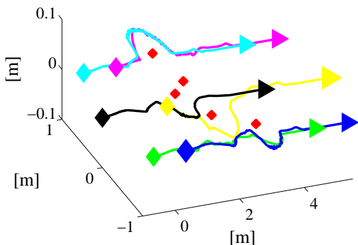
Fig. 4. Trajectory for each agent in the 3D space. Each color identifies an agent. The coloured diamonds are the initial positions of each agent’s path, while the coloured triangles are the arrival points. Red diamonds are the considered obstacles.
