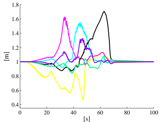
Fig. 3. Time history about the distance of each agent from the center of the swarm. Each color identifies an agent. The threshold \sigma_t over than an agent is considered lost has been not depicted in this plot.
