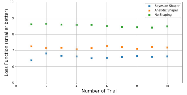
Fig. 9. Comparison of residual vibrations.
